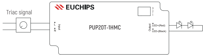
Wiring Diagram
